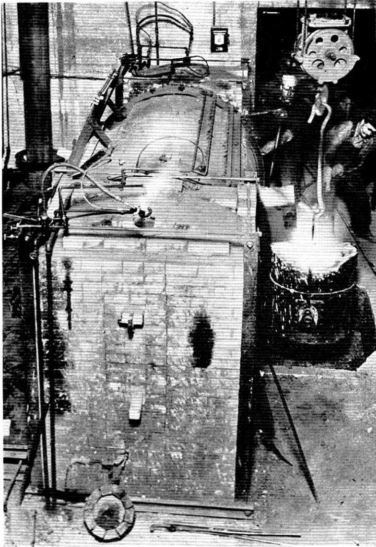
FIG. 2—HALF-TON TILTING OPEN-HEARTH FURNACE.
